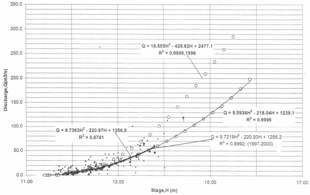
Stage-Discharge Curve of Pondok Tanjung
