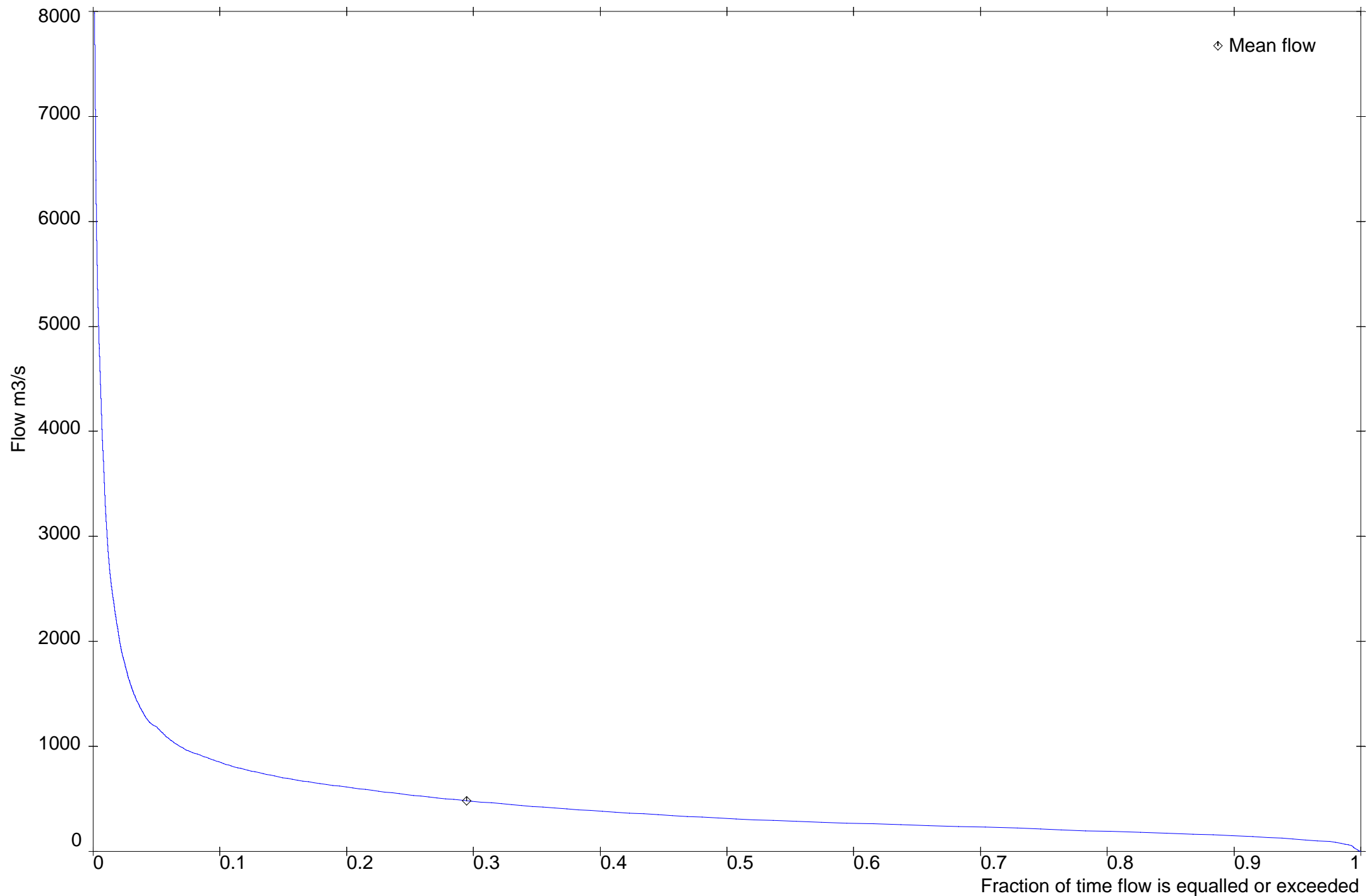
— site 5721442 SG. KELANTAN at JAM.GUILLEMARD, Kel. Flow m 3 /s 19600701 030000 to 20130923 101505
