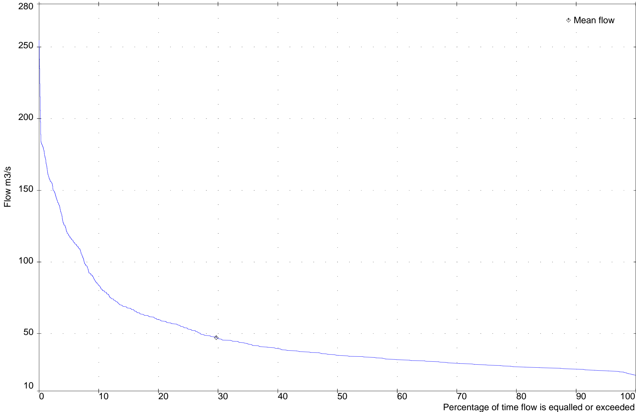
— site 5505412 SG. MUDA at LDG.VICTORIA, P.PINANG Flow m3/s 1-Jan-2013 00:00:00 to 31-Dec-2013 24:00:00
