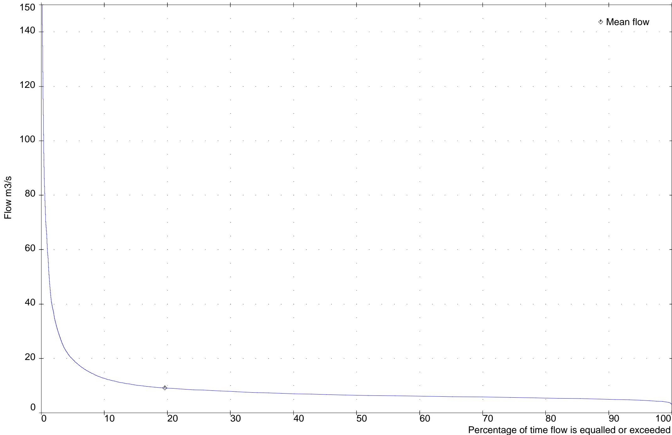
— site 2917401 SG. LANGAT at KAJANG,SELANGOR Flow m3/s 1-Jan-2013 00:00:00 to 31-Dec-2013 24:00:00
