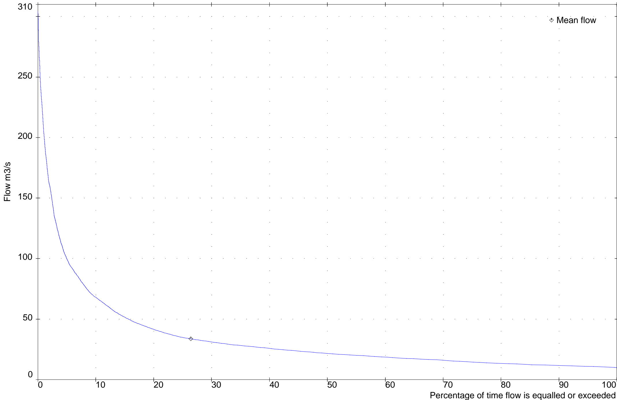
— site 2816441 SG. LANGAT at DENGKIL,SELANGOR Flow m3/s 1-Jan-2013 00:00:00 to 31-Dec-2013 24:00:00
