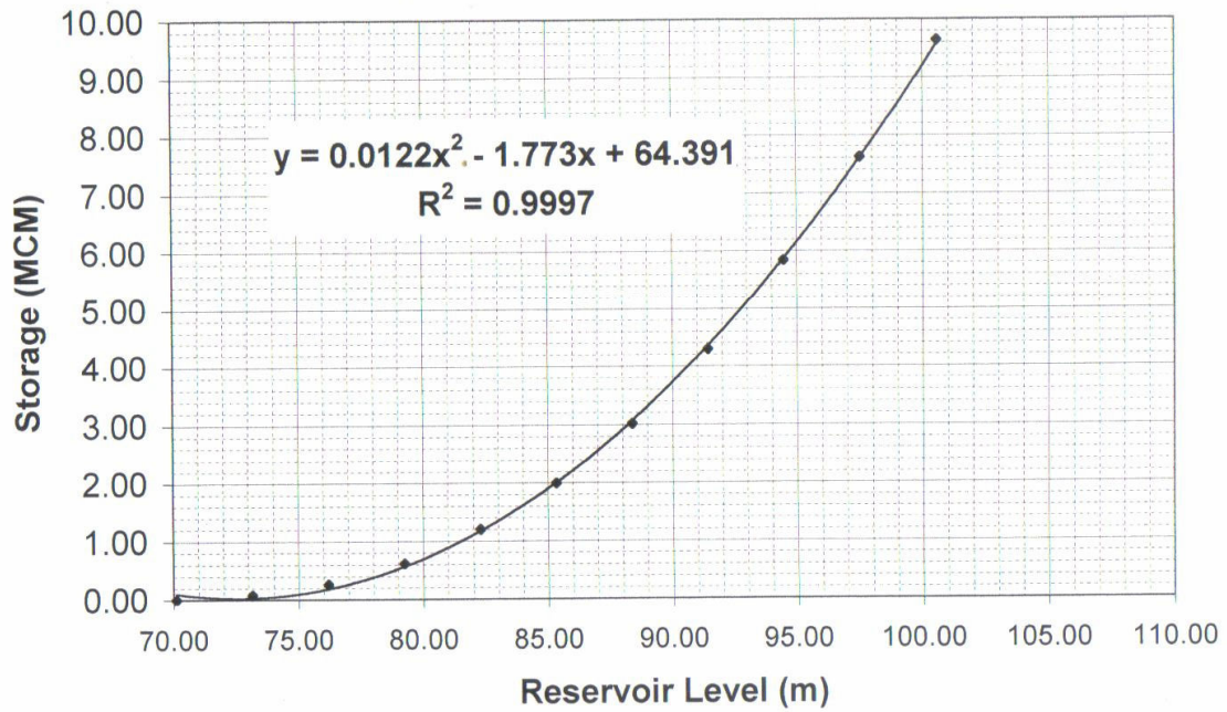
Klang Gate Dam vs Stage - Storage Curves. (Source : July, 1987 )
